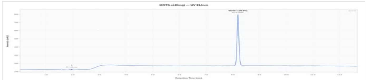
MOTS-C 40mg - MS-001: UV Chromatogram
