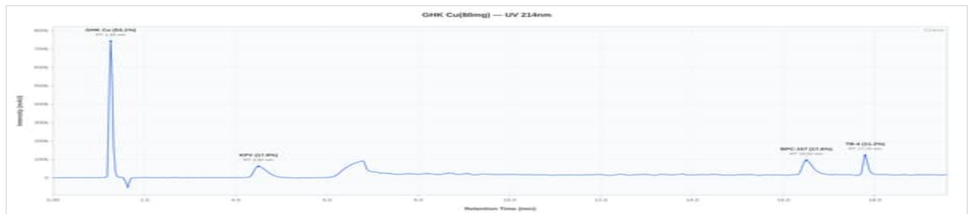
GHK-Cu / TB-500 / BPC-157 / KPV 80mg - KLOW-001: UV Chromatogram
